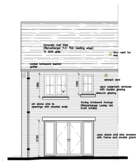
Rear Elevation
