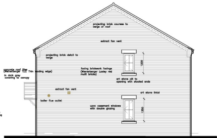
Gable Elevation
