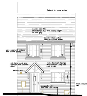
Approach Elevation
